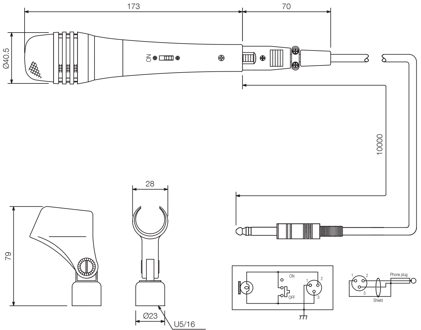
Circuit Diagram
