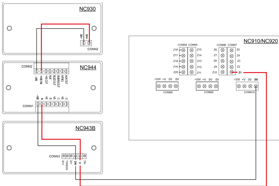
Fig. 1 – Wiring Connections
