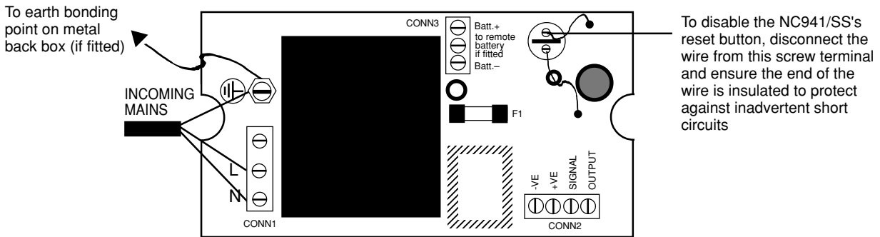
Figure 1 : NC941/SS PCB LAYOUT
